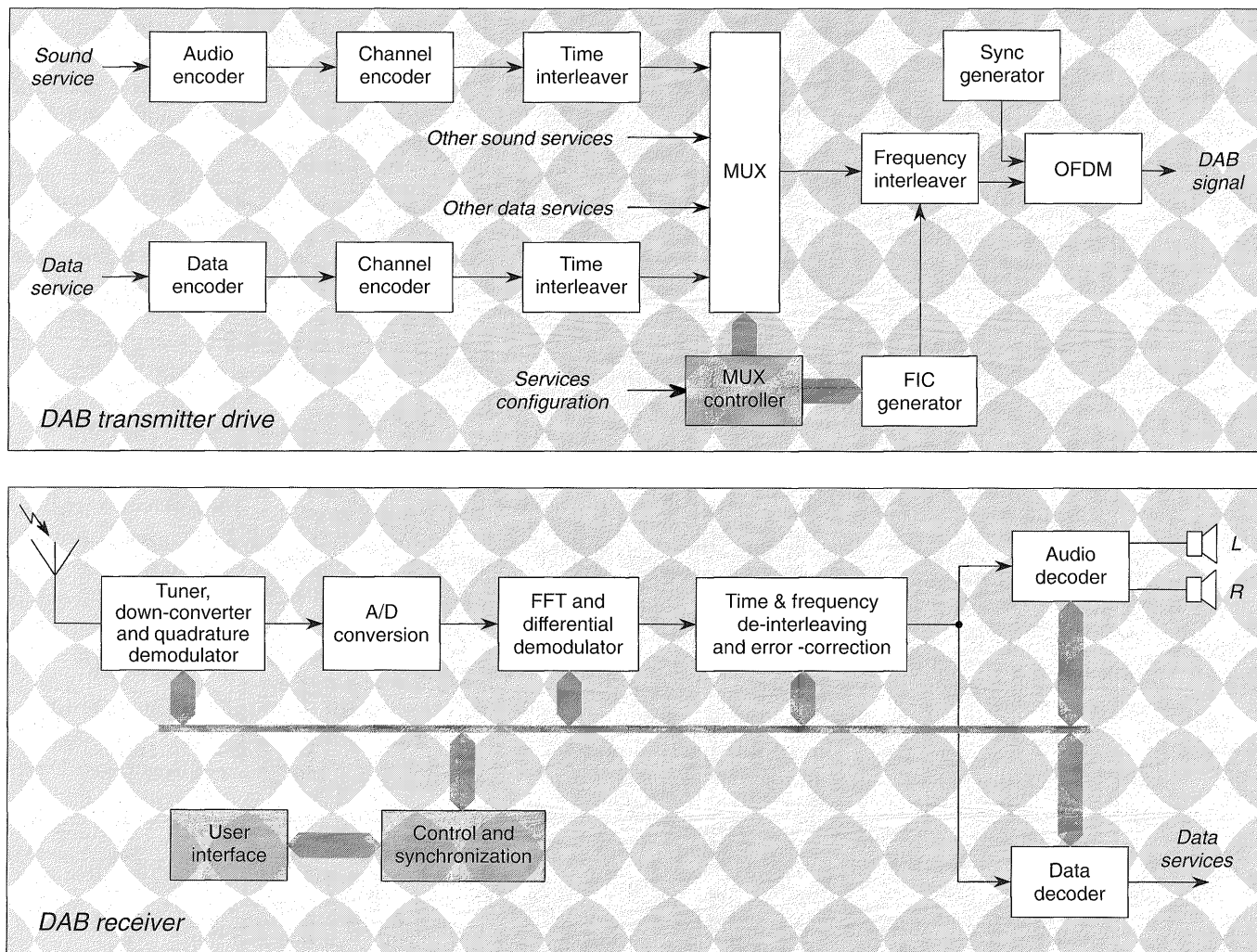
Figure 1 Conceptual DAB transmitter drive (top) and DAB receiver.
